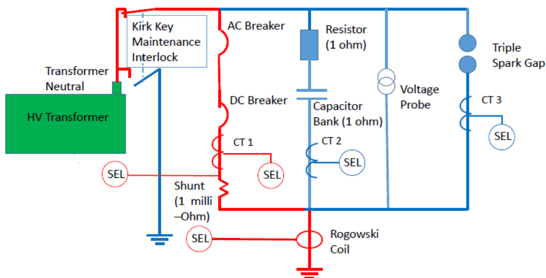
Figure 9: Neutral Blocking Device (SolidGround™) Circuit Diagram.
