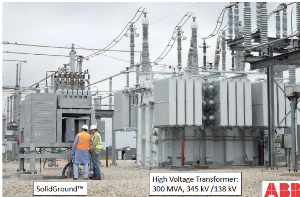
Figure 8: SolidGround™ Neutral Blocking Device Installed and Operational in Wisconsin.
