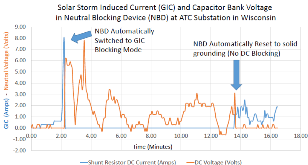
Figure 11: Recording of Neutral Blocking Device (NBD) June 22, 2015, Automatic Operation. Blue Trace is GIC Current (amps) and Orange Trace is Capacitor Bank Voltage (volts).
