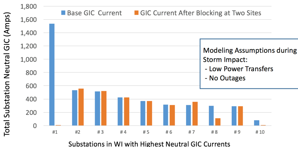
Figure 5: Modeled GIC Before (Blue) and After (Orange) Neutral Blocking added at Sites #1 & #10 for a Severe (19 V/km) GMD at Worst Field Angle (W to E). Little to no GIC “Whack-a Mole.”
